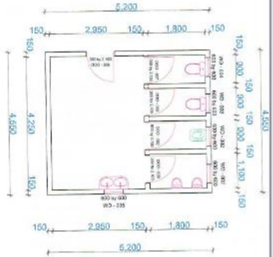
FLOOR PLAN - WASHROOM
